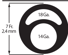
Catheter Cross Section
