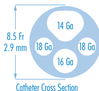
Catheter Cross Section
